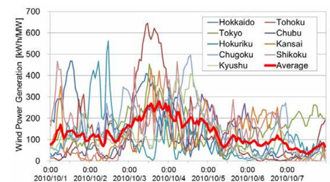
Variation of Wind Power Generation
