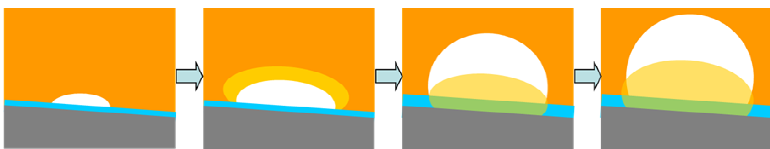
Formation of small cavity due to erosion at some point Erosion progressed. Cavity and surrounding loosened area expand Failure of cavity ceiling By repetition of erosion and failure of cavity ceiling, a cavity moves upward
