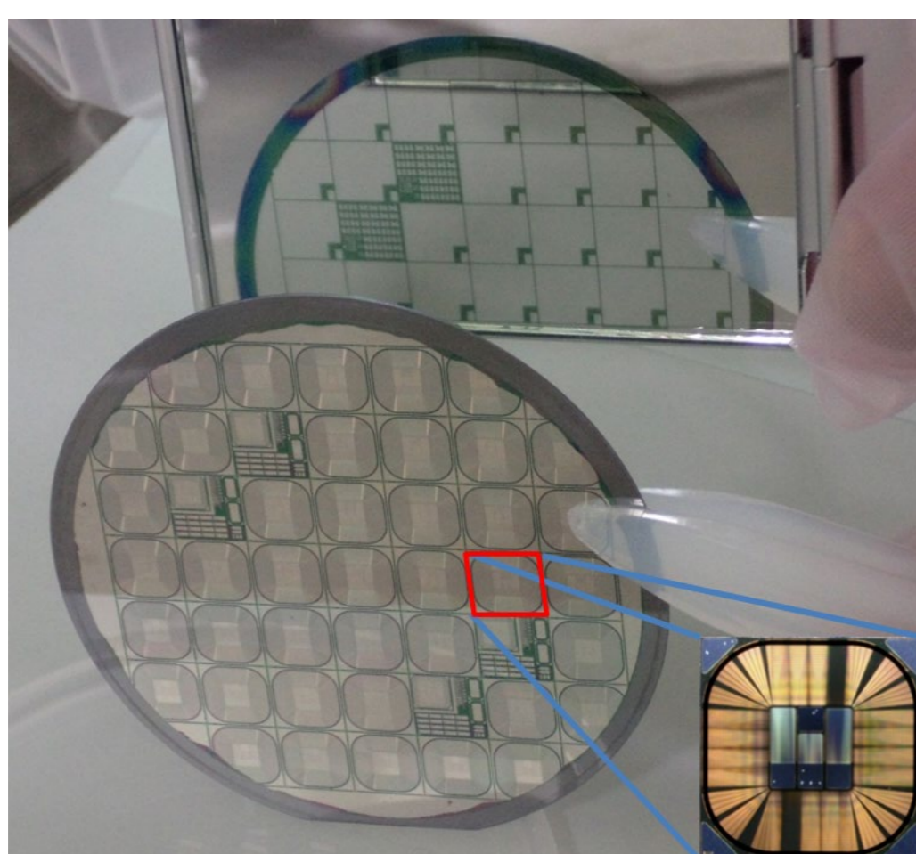
Fig. 2. The silicon power device project was initiated. The current density of IGBT was improved by the scaling concept at blocking voltage of 3000V. The double-gate IGBT was also demonstrated.
