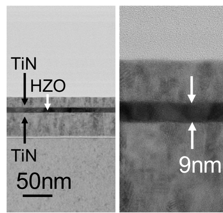
Fig. 3. CMOS-compatible ferroelectric nano film is an enabler for ultralow power logic and memory technology.
