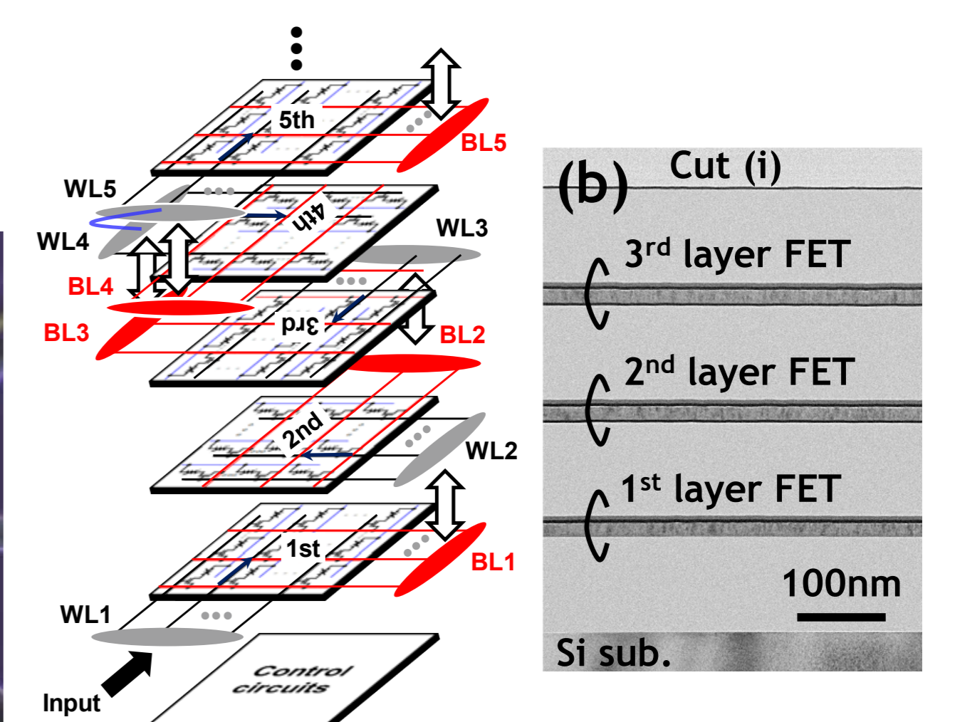
Fig. 5. 3D integration technology by oxide semiconductor IGZO transistor for AI hardware.
