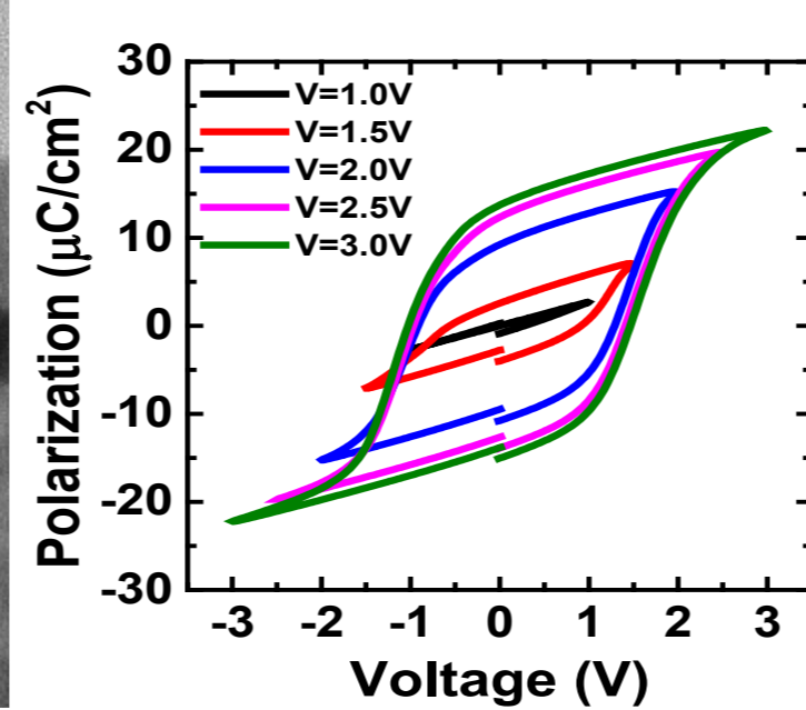
Fig. 3. CMOS-compatible ferroelectric nano film is an enabler for ultralow power logic and memory technology.
