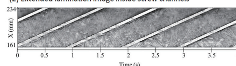
長繊維強化樹脂可塑化過程の可視化解析 Visualization analyses of plastication process of long-fiber reinforced resins
