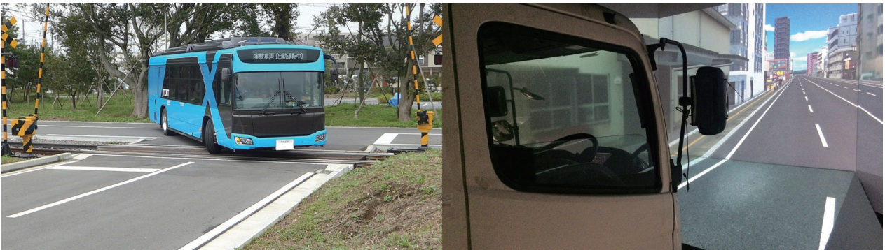
大型車の自動運転・運転支援の実験 Experiment of automated driving and driving assistance for a large vehicle.
