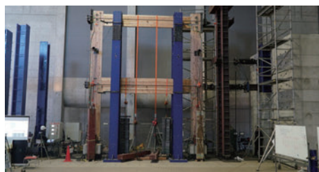
静的載荷関連設備および反力壁 Static loading related facilities and reaction wall
