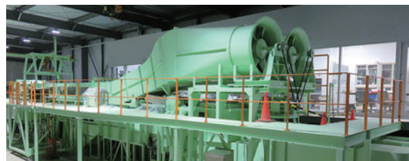
海洋工学水槽と風路付き造波回流水槽 IIS Ocean Engineering Basin and Circulating Water Channel
