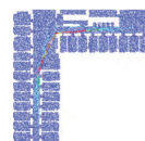
Betweenness centrality
