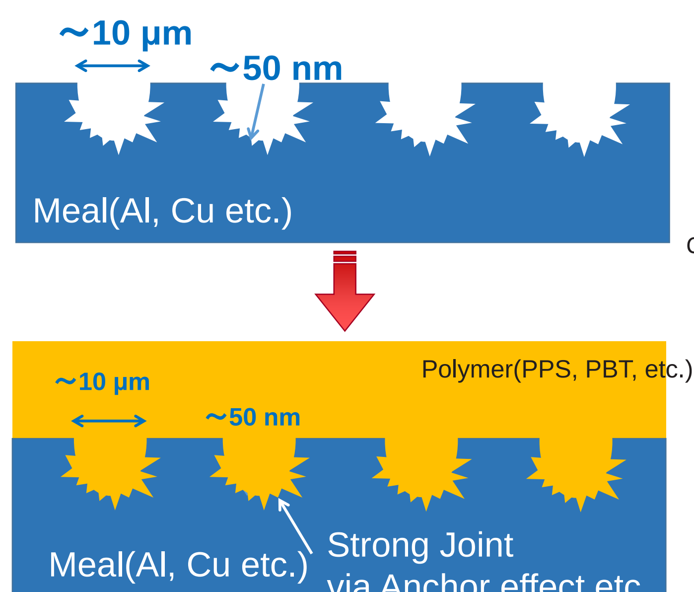
Concept of direct joining
