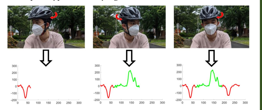
Figure 2. Rider made three head movement sequences and the corresponding data of gyroscope z axis.
