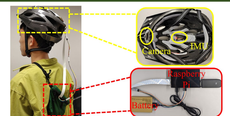
Figure 1. Participant wearing the helmet prototype and carrying the accessories.
