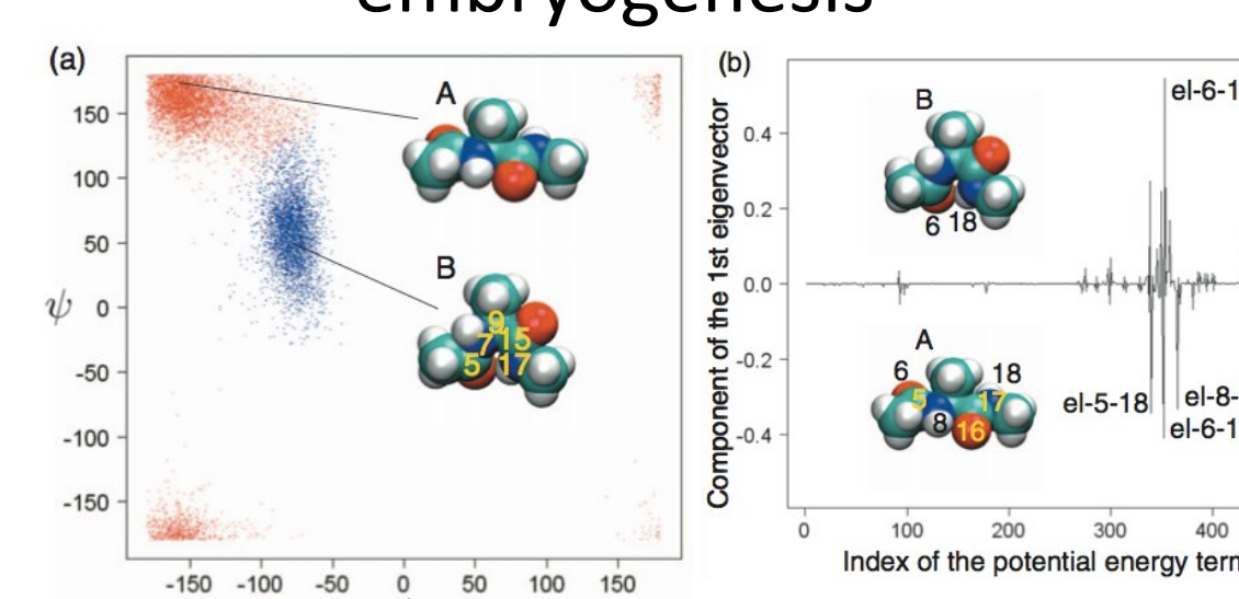
Fig. 3 Potential energy PCA analysis of peptide folding
