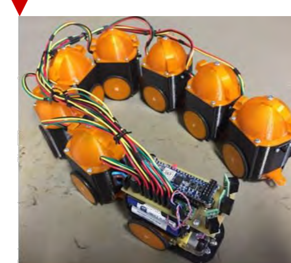
Snake robot
