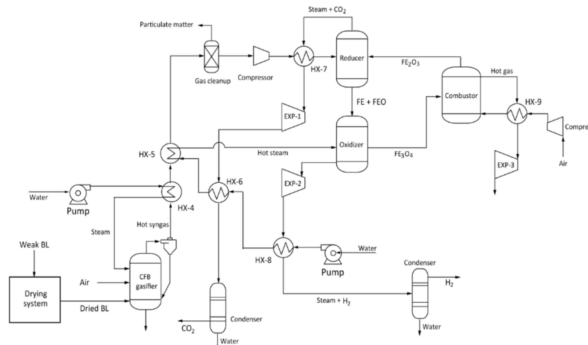
Highly efficient hydrogen production system utilizing industrial wastes
