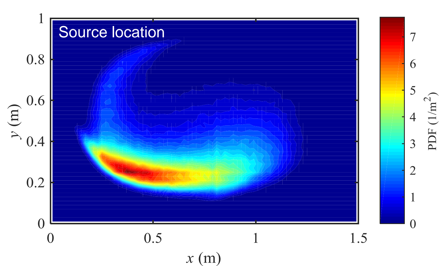
Inverse analysis of pollutant source parameters
