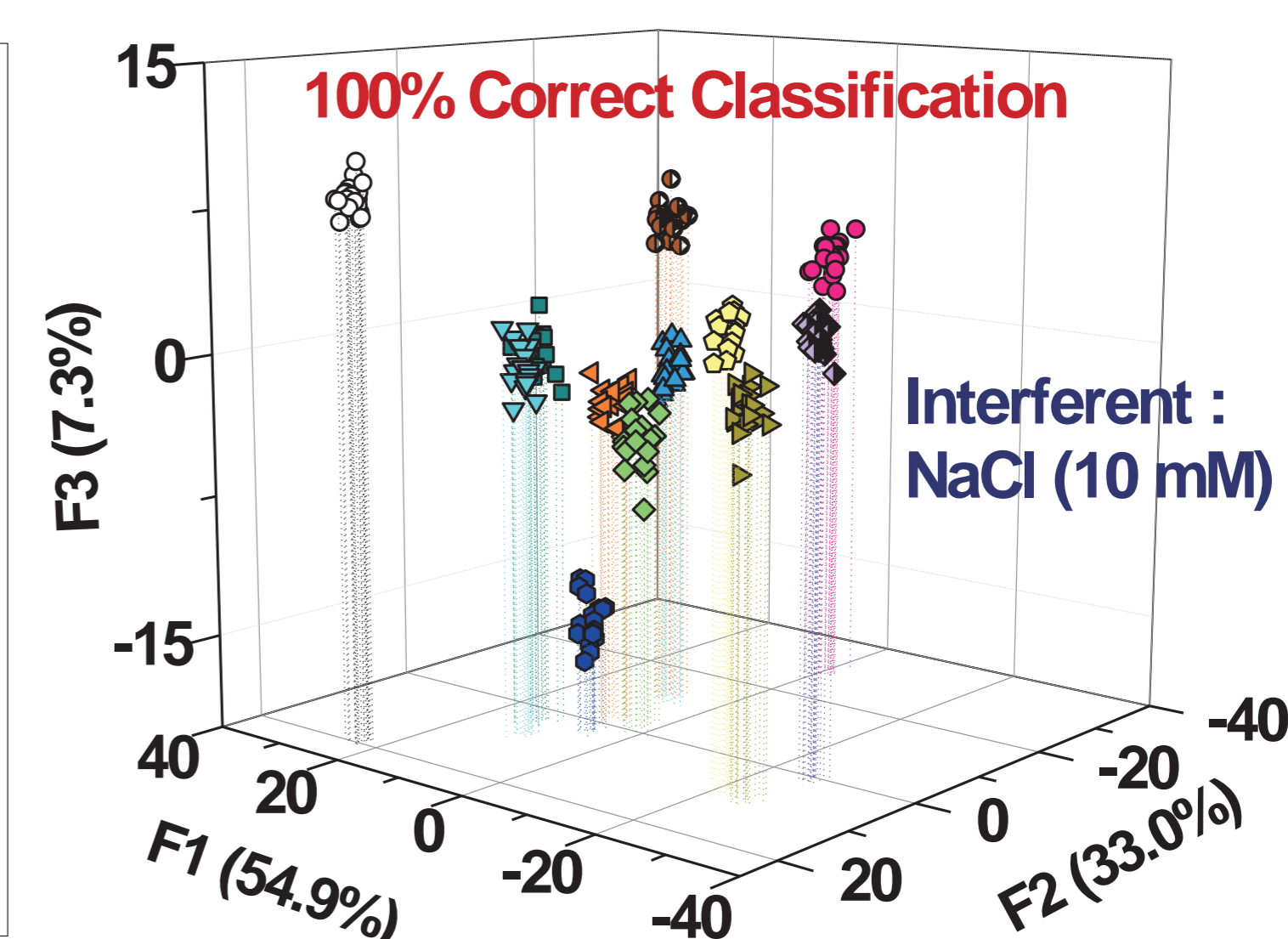
Ex. : Molecular self-assembled colorimetric chemosensor array for simultaneous detection of metal ions
