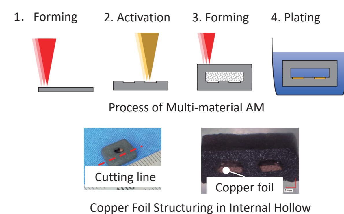
Copper Foil Structuring in Internal Hollow
