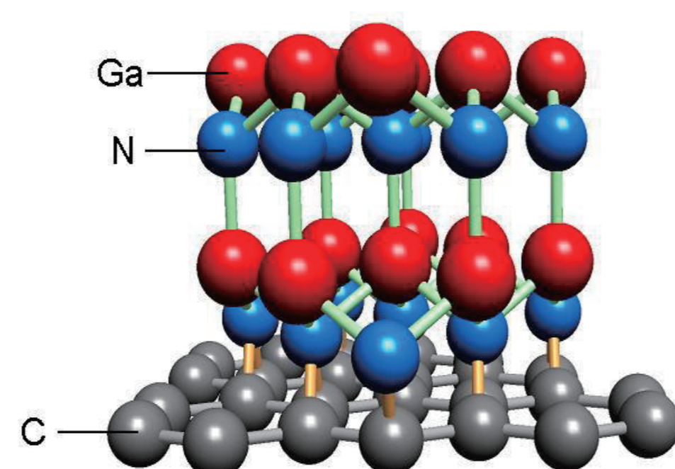
A schematic illustration of the atomic arrangement at the hetero-interface between GaN and graphite
