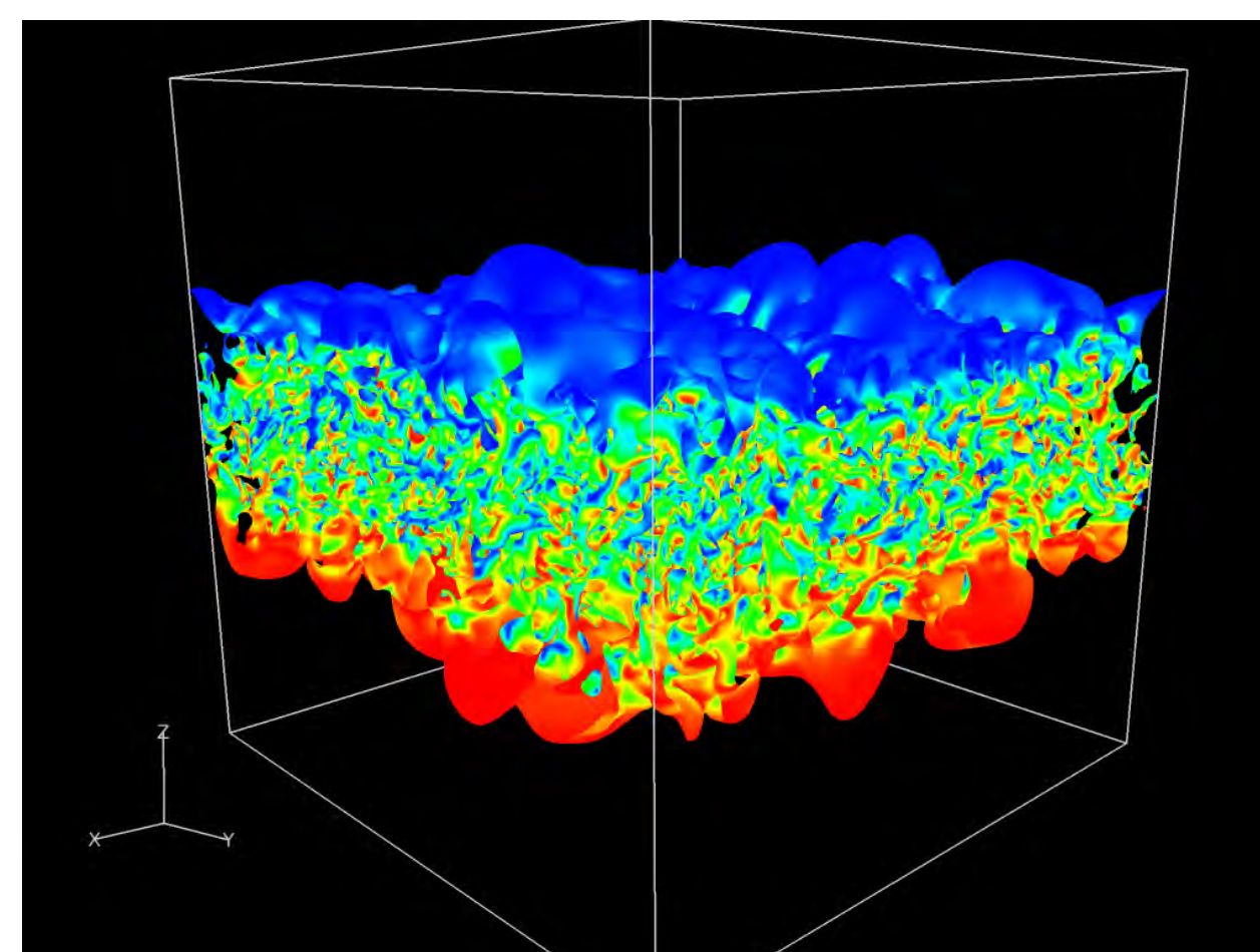
Fig.2 Kinetic energy of turbulent diffusion in a rotating system
