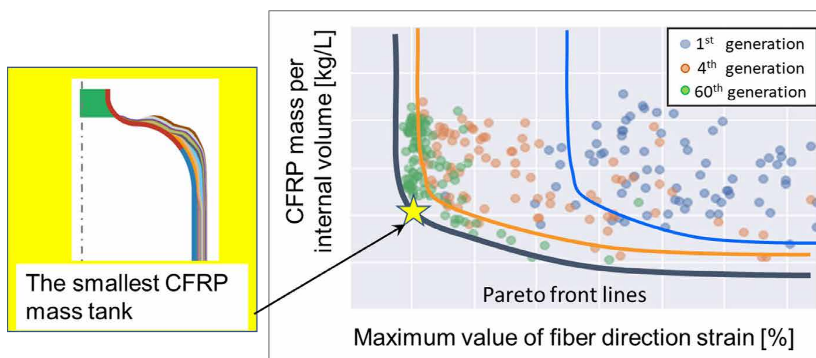
Mesoscale model simulation of high pressure hydrogen tank
