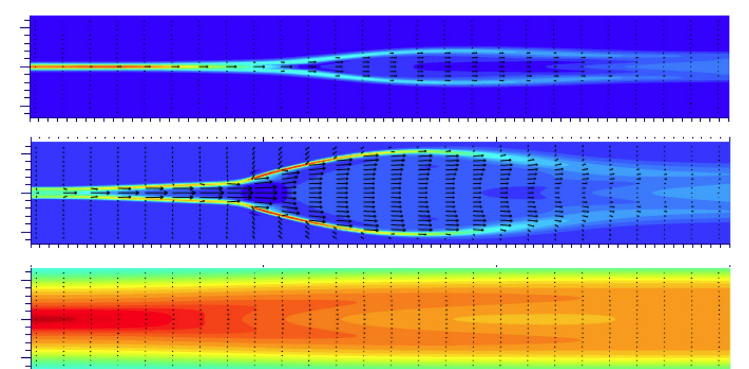
Fig.3 Jet and electric current of magnetic reconnection
