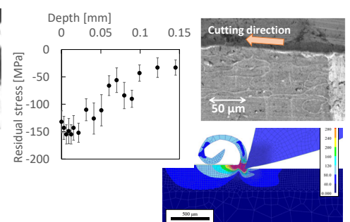
(Upper left) Residual stress distribution of the workpiece, (Upper right) Crystal structure inside, (Lower right) Stress distribution analysis result during cutting
