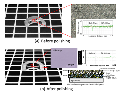
Fixed micro abrasive tool with super long life.
