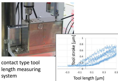
Repeated test of tool contact detection
