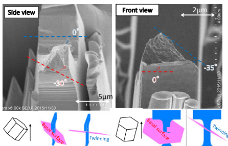
Fatigue test under real-time observation.
