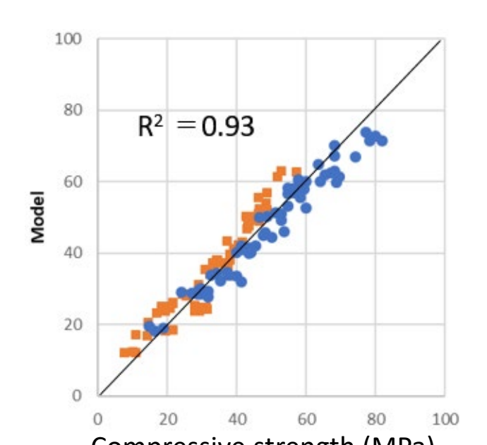
Compressive strength estimation
