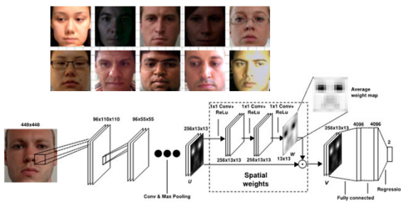
Deep Learning-based Gaze Estimation
