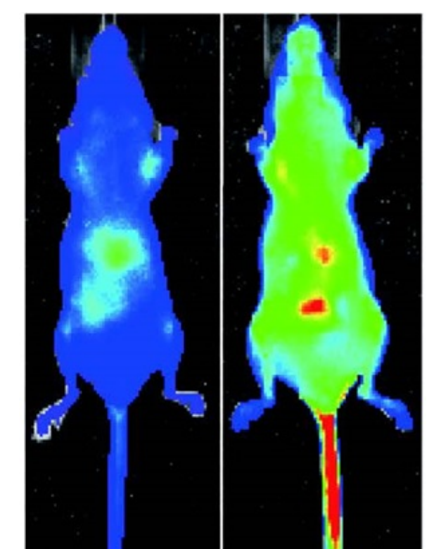
Fluorescent imaging of Vitamin C in a mouse
