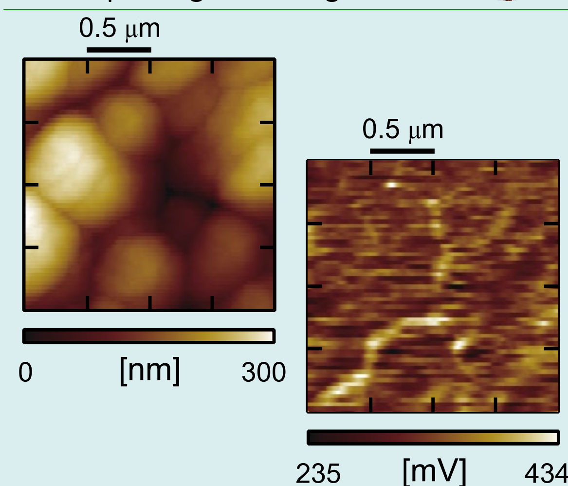
Images of topography (left) and photovoltage (right) on Cu(In,Ga)Se 2 solar cell
