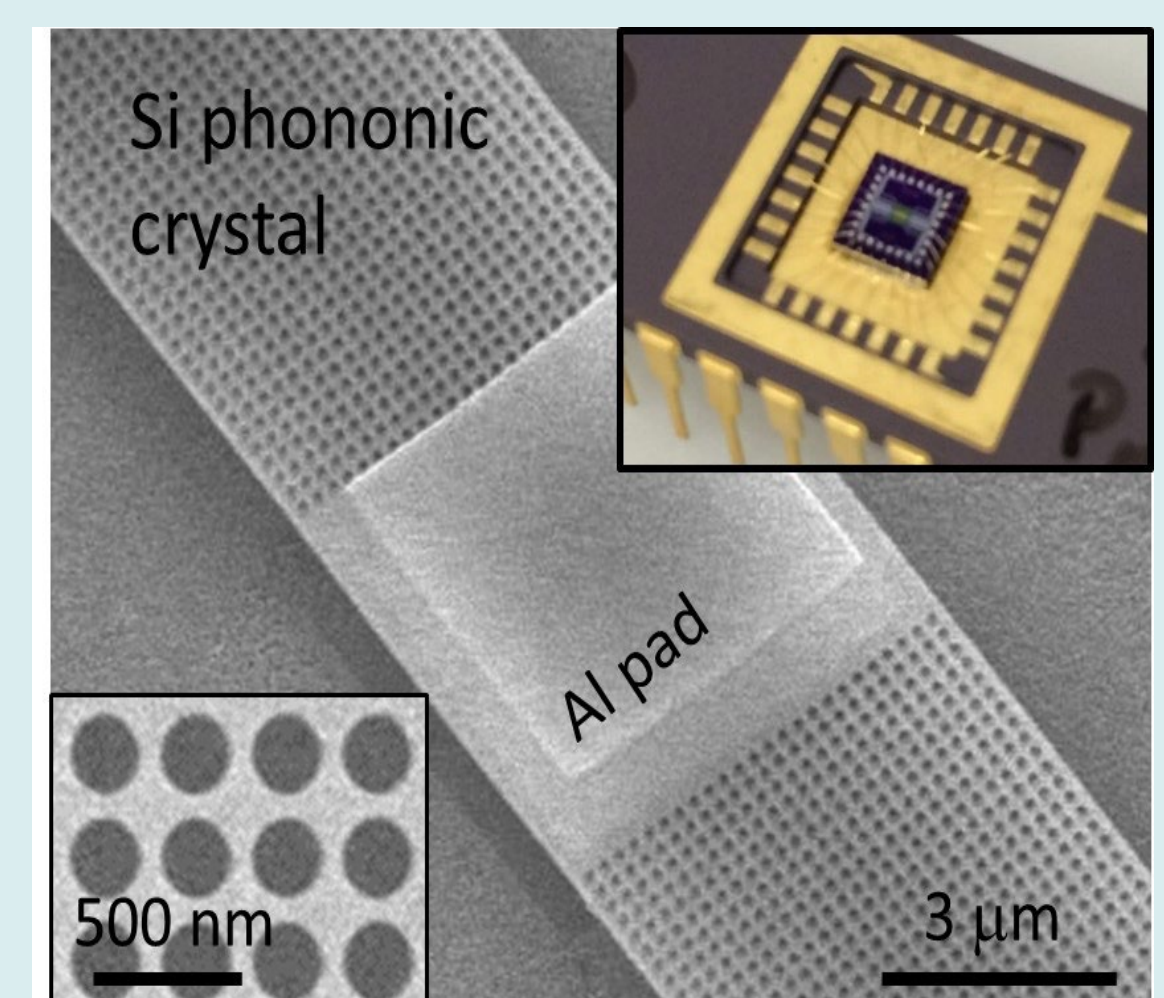
Nanostructured Si thermoelectric energy harvester
