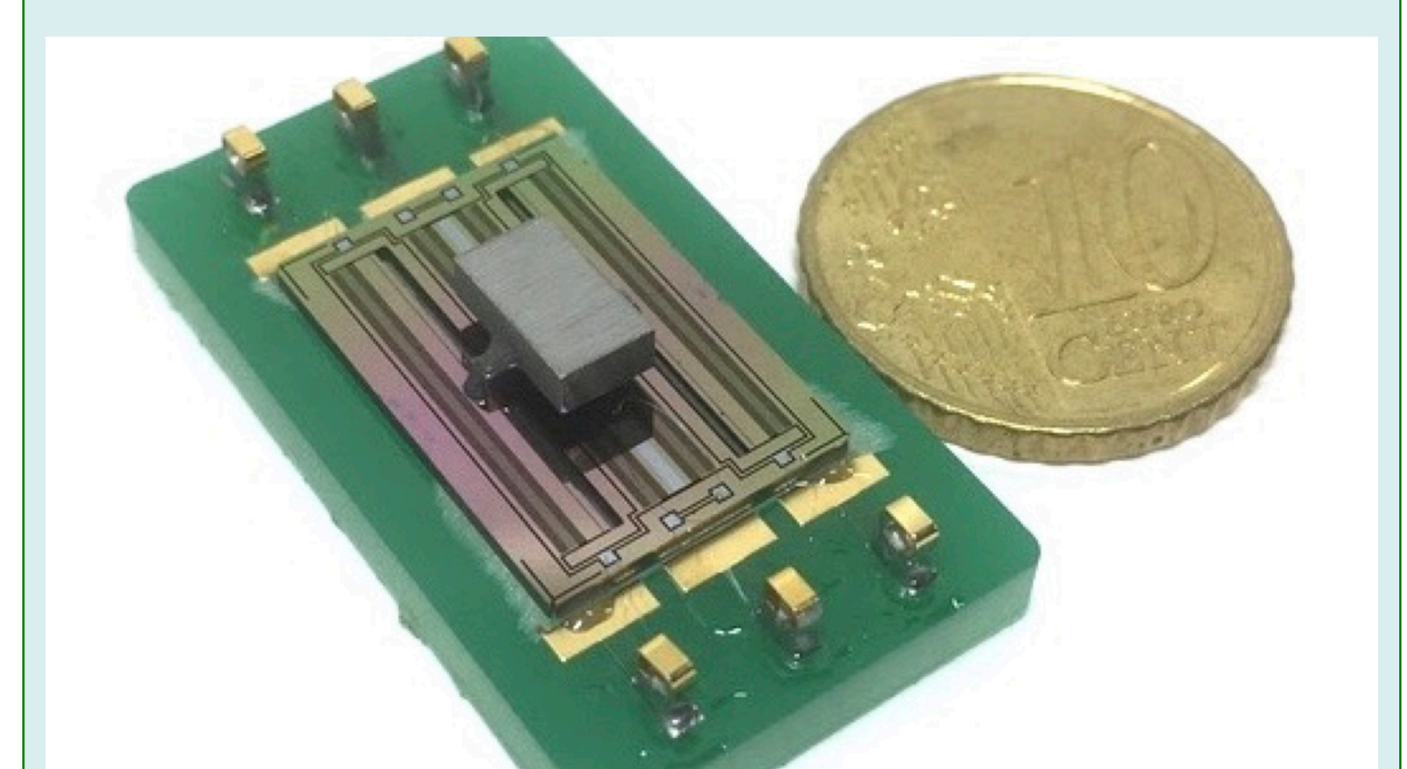
MEMS environmental vibrational energy harvester
