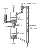
CO 2 -free hydrogen production system
