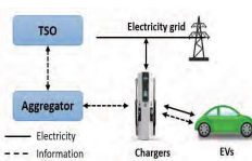
Basic configuration of VGI
