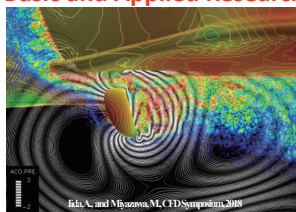
Flow and resulting sound around side mirror
