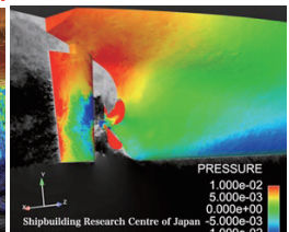
Flow around ship
