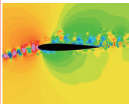
Sound radiated from turbulence
