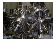
Variable temperature SPM in ultra-high vacuum
