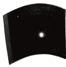
Luminescence from GaN grown on graphite sheets
