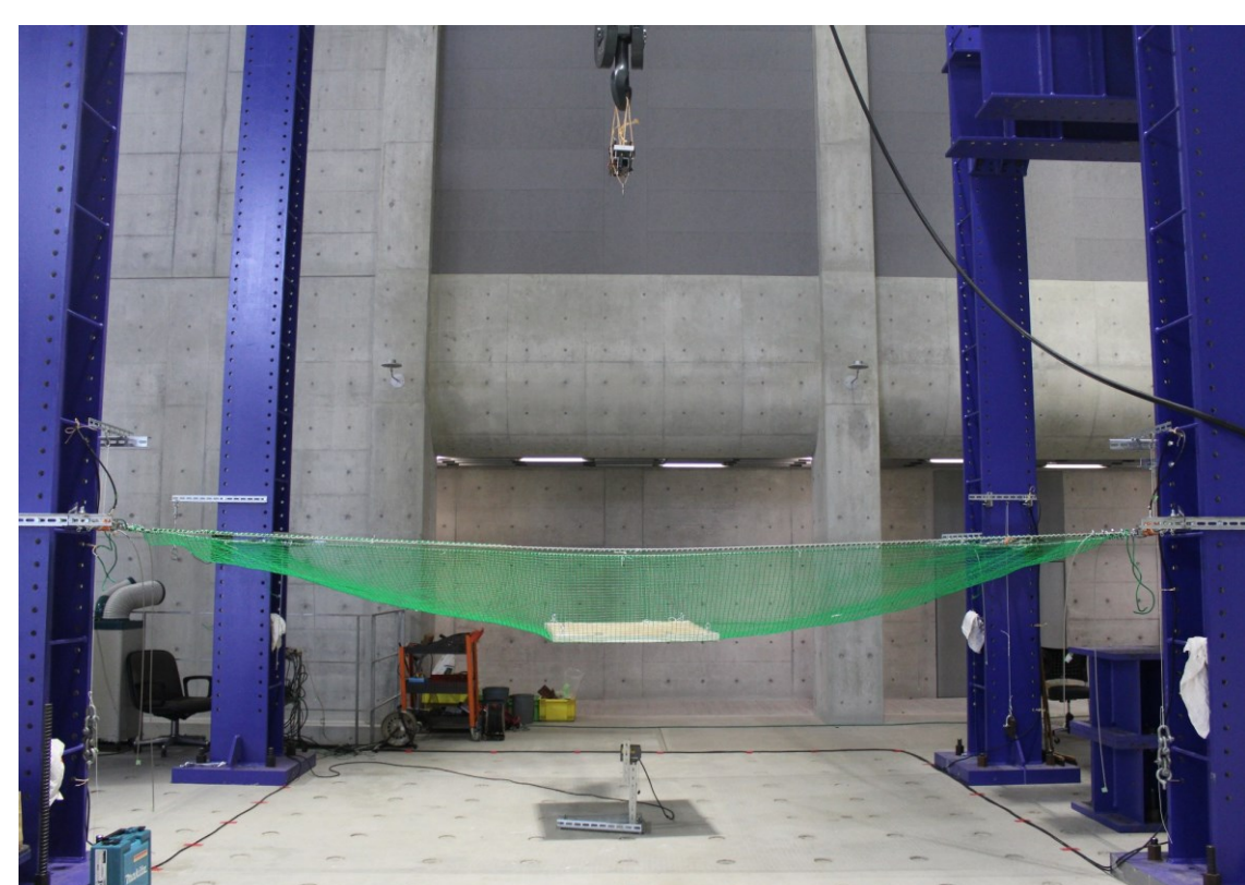
Real-scale tests of the safety net
