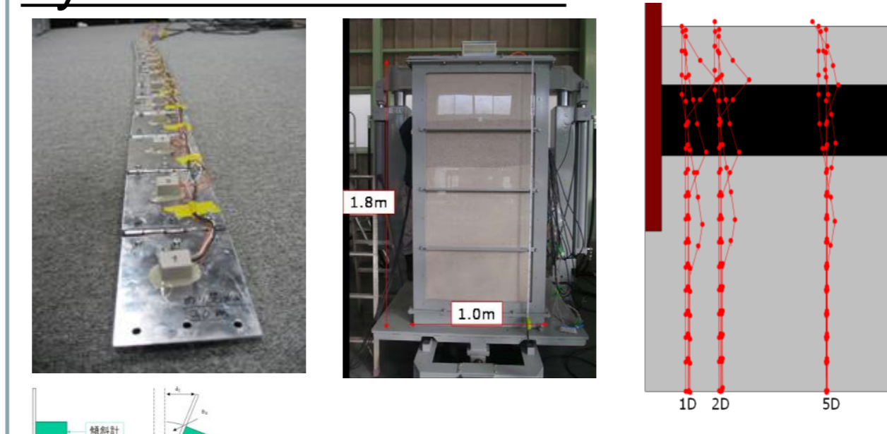
Measure the soil deformation during the press-in execution.
