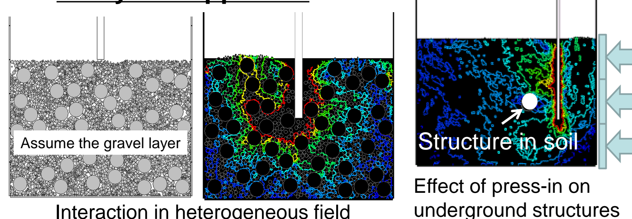
Measure the soil deformation during the press-in execution.
