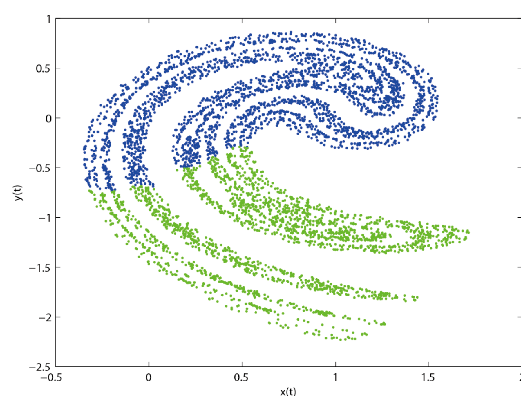
Fig. 2. Noisy Ikeda map partitioned into two in such a way that the information related to dynamics is maximally preserved. (ref: Hirata and Aihara, Eur. Phys. J. Spec. Top. (2013))
