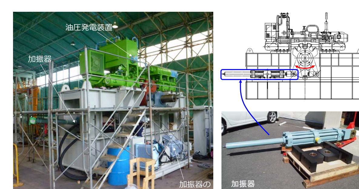
Experimental full scale test bed of wave energy converter
