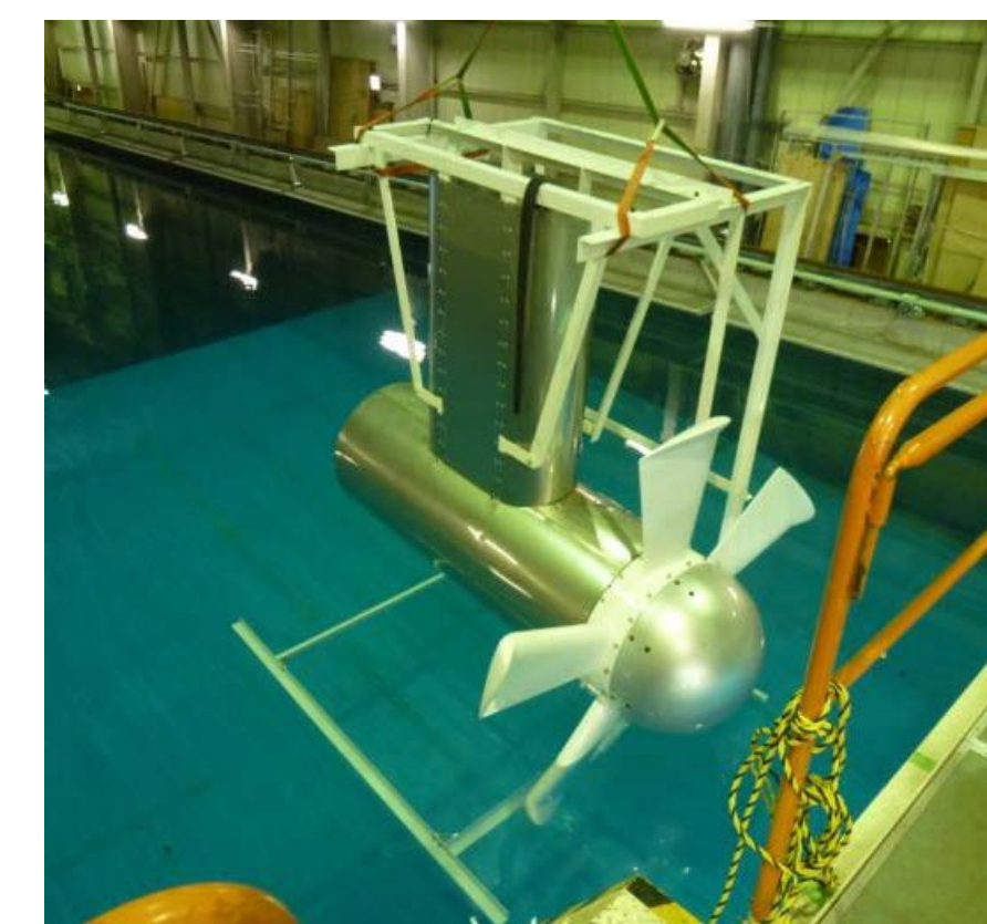
Rotor test in water tank
