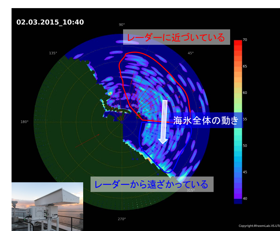
Sea ice observation using microwave Doppler radar
