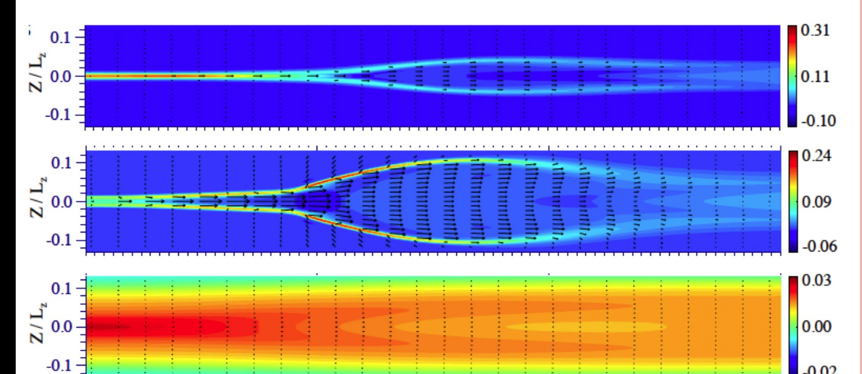
Fig.3 Current and jet of magnetic reconnection
