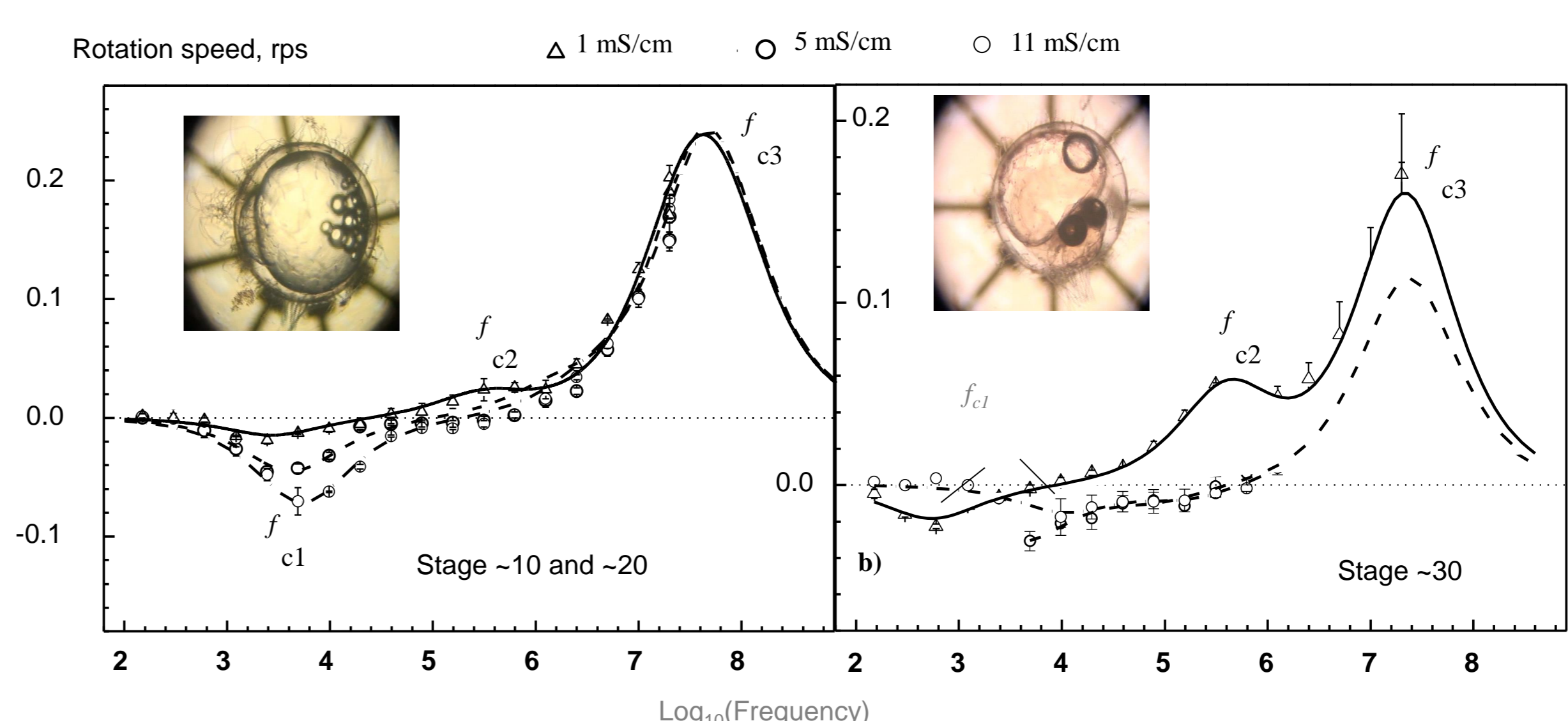
Fig.3 Electrorotation spectra of single fish egg
