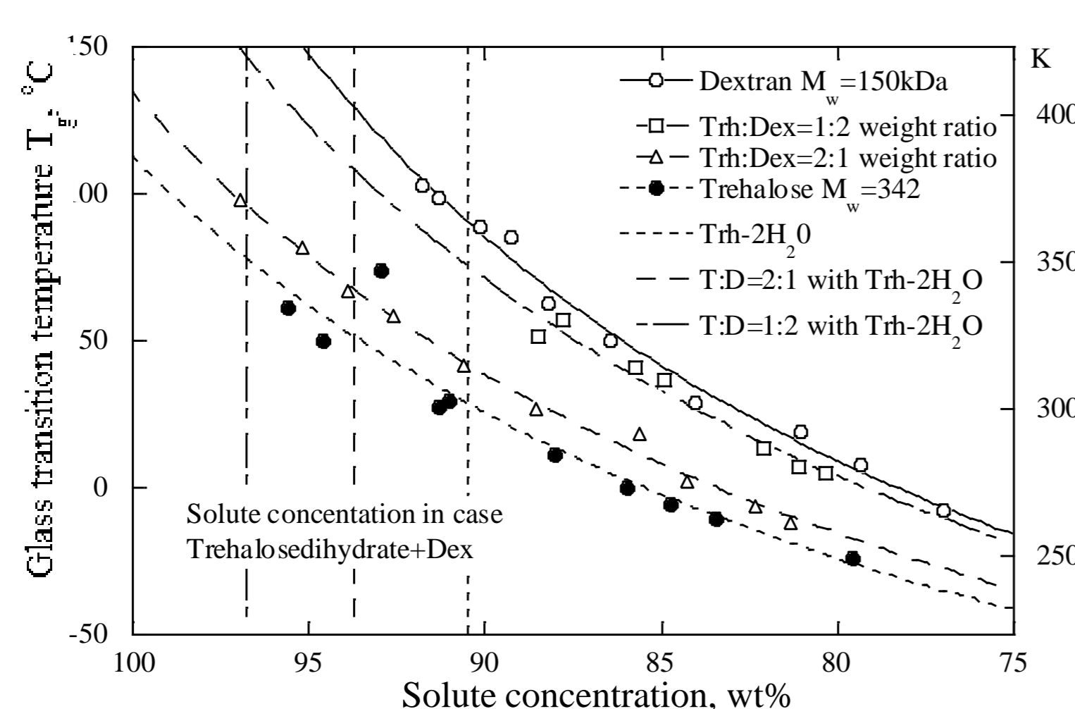
Fig.1 Glass transition diagram of protective agents
