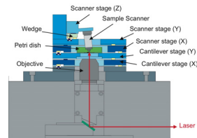
AFM for in Liquid Measurements
