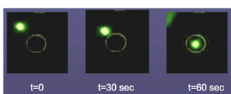
in vitro Reaction Networks for Complex Behaviors
