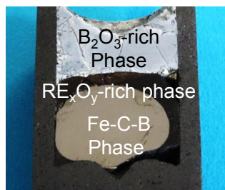
3 phase separations of the RE(Nd, Dy, Pr)-Fe-B-C-O system
