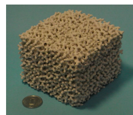
Fabrication of photonic amorphous diamond structure in a microwave regime
