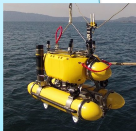
AUV Tri-TON
