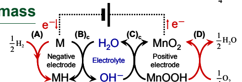
Schematic image of Fuel Cell/Battery System (upper) discharge (lower) charge
