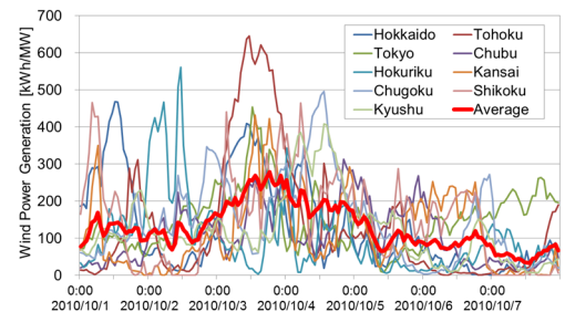
Fig. Variation of Wind Power Generation
