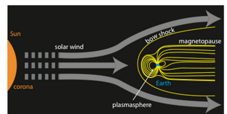
Fig.3 Solar wind and Earth's magnetic field
