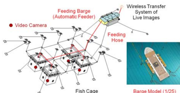
Offshore underwater aquaculture system
