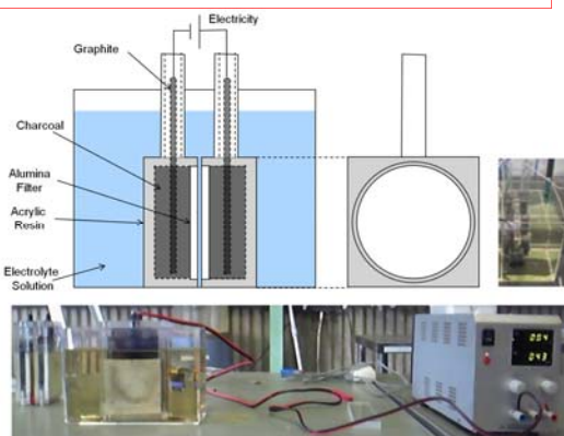
Treatment of wastewater by electrolysis
