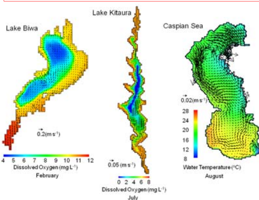
Future prediction of the ecosystem of lakes and coastal seas by hydrodynamic and ecosystem coupled model
