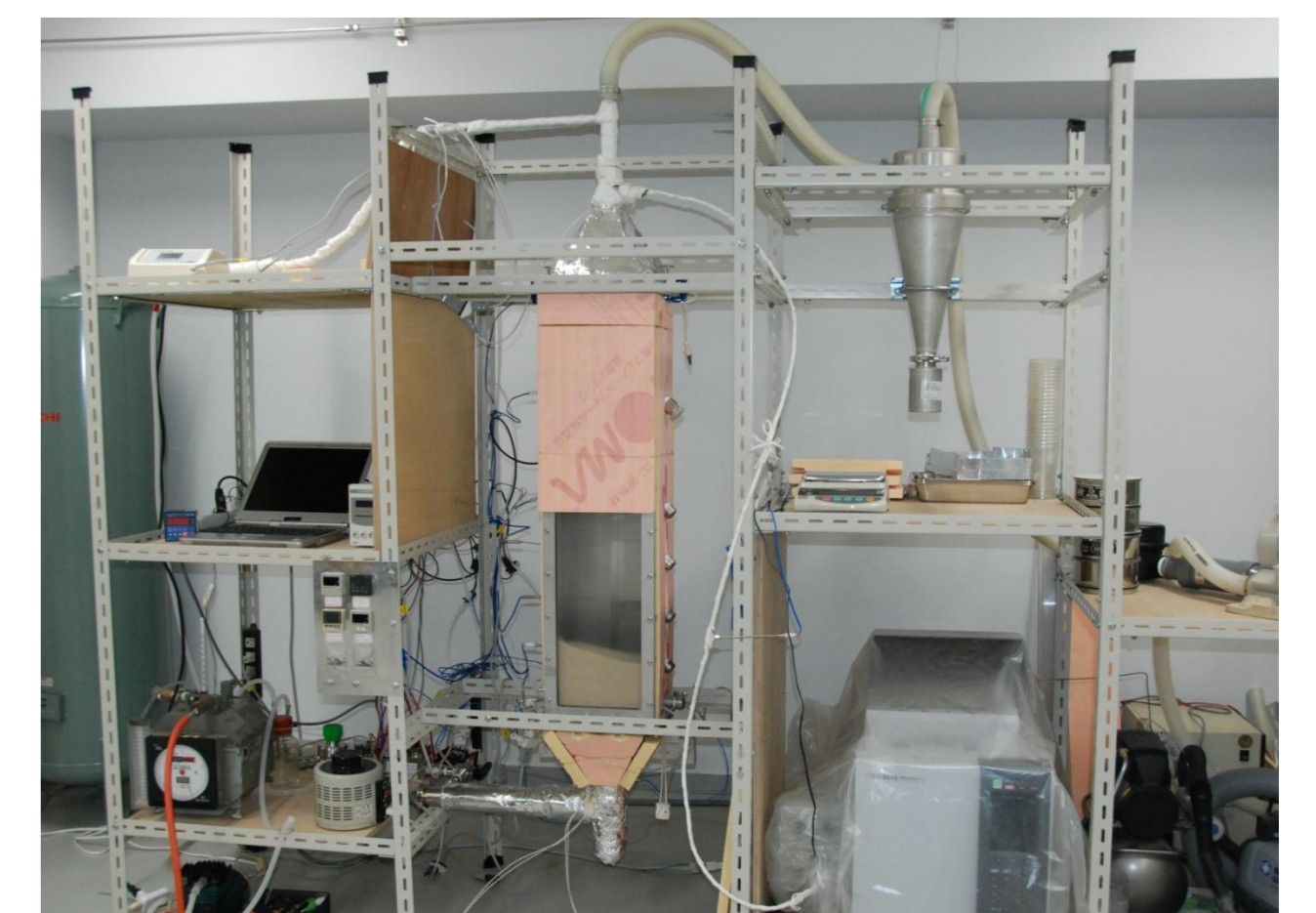
Fluidized bed dryer
