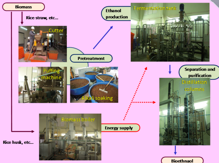
Small-scale bioethanol system for biomass town
