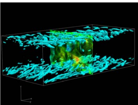
Fig.1 Vortices near the walls in turbulent channel flow
