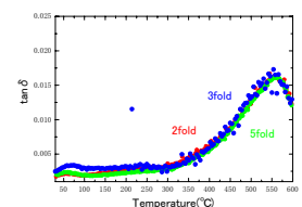
Measurement of high-temperature internal friction
