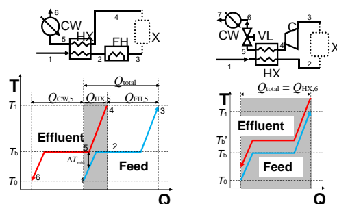
Schematic image of conventional heating process (left), and self-heat recuperation (right)
