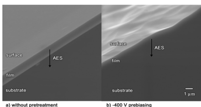
Cross sectional SEM images of DLC/Si interface. No clear interface between the substrate and the DLC film are identified in the film (b) deposited after a negative biasing to the substrate.
