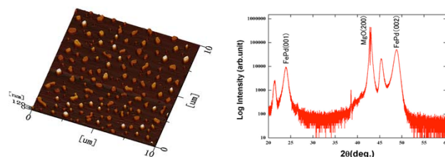
FePd nanodots with diameters of a few tens of nm were formed through the deposition of Fe seeding layer and Au agglomeration layer on a single crystalline MgO substrate. AFM image and X-ray diffraction pattern show oriented crystals and an uniform size of the FePd dots.
