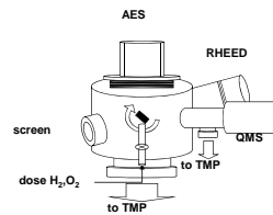
Schematic diagram of the surface analysis chamber. The base pressure < 10^{-9} Pa is achieved inside the chamber. AES, RHEED, QMS and heated gas sources enable the surface modification and analyses of desorbed species
