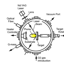
Pulsed-laser deposition chamber with a Nd-YAG laser. The base pressure reaches 10^{-7} Pa, reducing unwanted impurities.
