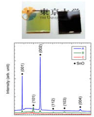
Oriented crystalline of SnO films were achieved on a glass by controlling oxygen and Sn flux during the film deposition.
