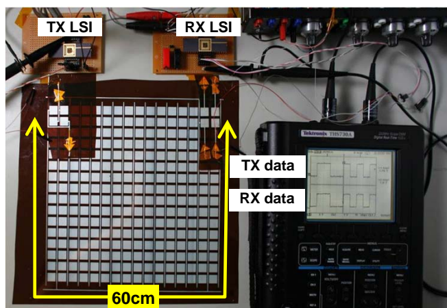
communication sheet
