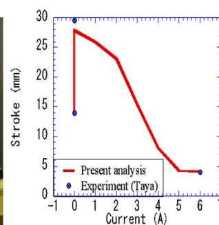
Magneto-superelastic response of FSMA actuator
