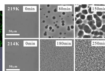
Process of liquid-liquid transition in triphenyl phosphite
