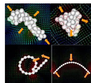
Flow field around a polymer undergoing a coil-globule transition
